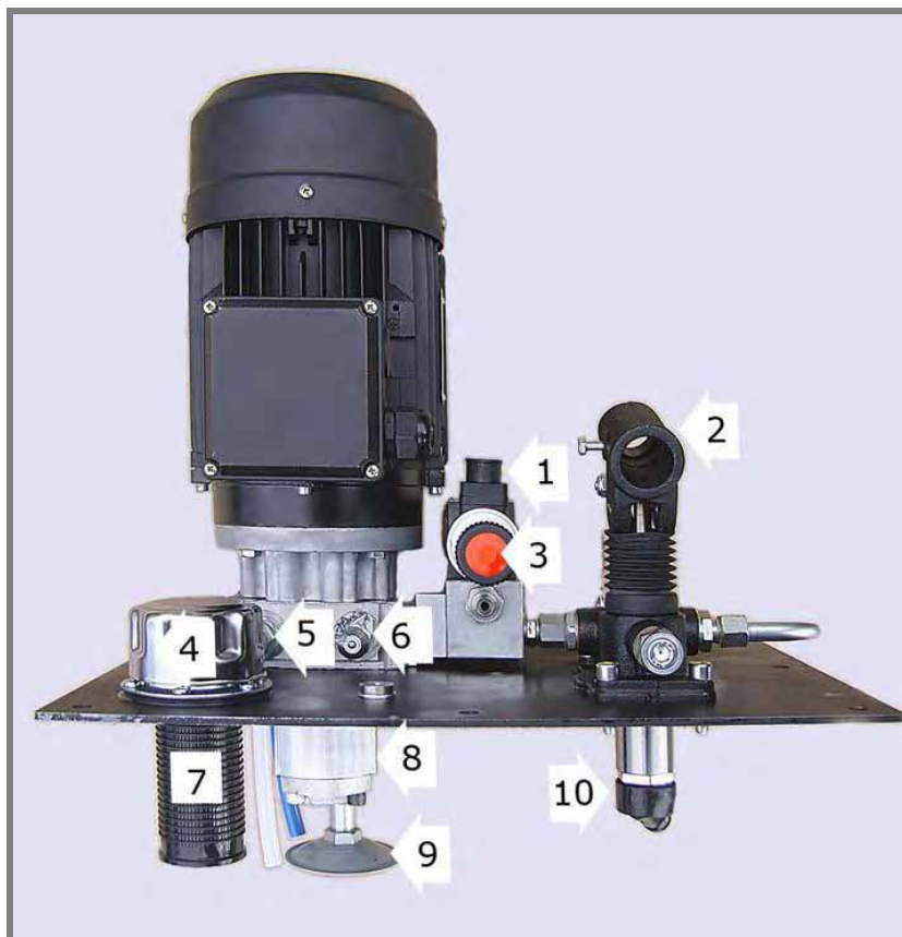
Illustration Hyd-002. Blocker/Barrier HPU.
