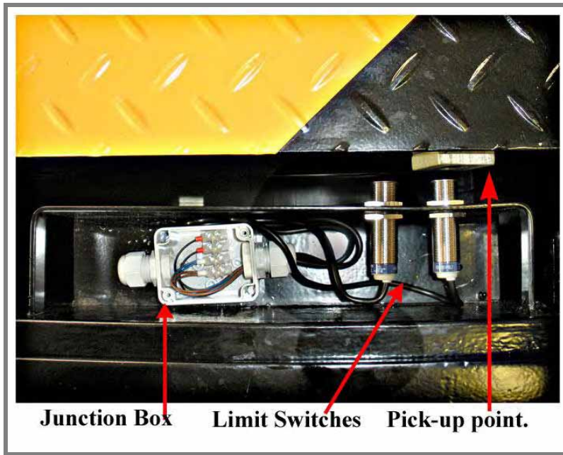
Illustration elec-003.Blocker limits
