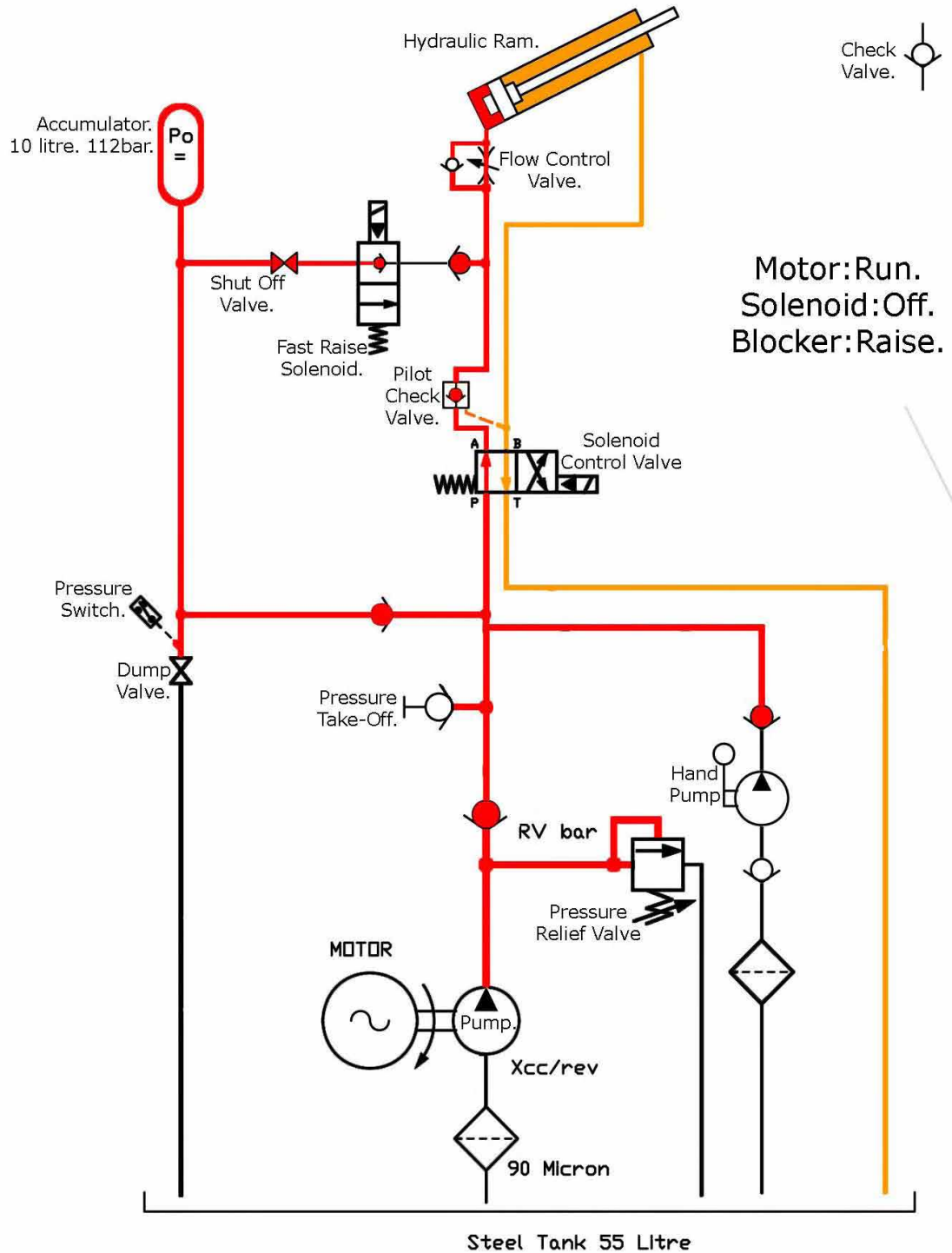
Illustration hyd-003. Blocker Accumulator Schematic.
