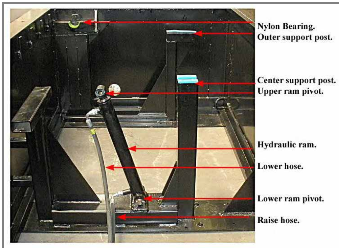
Illustration hyd.004 ram.
